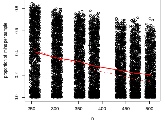
Figure 8: V6: Proportion of samples N/k holding the best answer S . Here n = 257, 304, 352, 383, 439, 470, 502 . We have k = 2000 (at n \leq 352 ), k = 5000 (at 383 \leq n \leq 439 ) and k = 10000 (at n \geq 470 ). The solid red line shows means and the dotted red lines shows medians.
