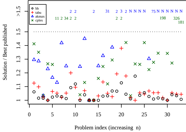
Figure 4: QAP relative solution quality. The y-axis is the ratio of solver solution to best published solution. Points above the line are not to scale (labeled by ratio); “N” denotes ten cases where AK failed to return a solution.
