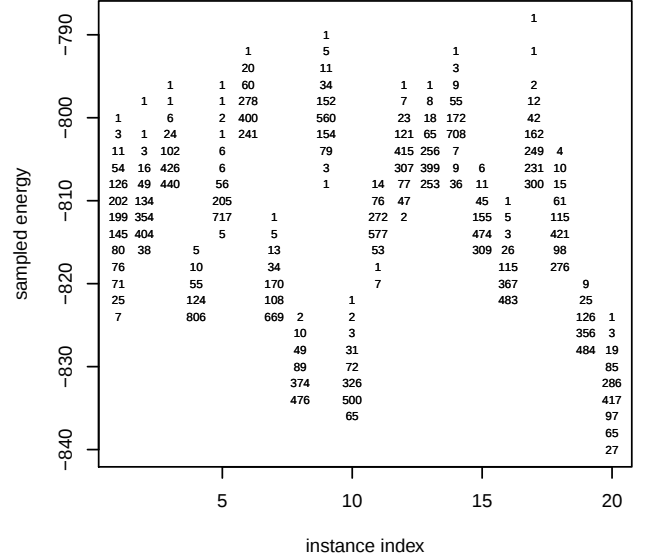
Figure 5: Distribution of V5 solution costs, n=439 , 20 instances. A number at position y gives the total number of samples (out of 1000) that returned solutions with cost y .
