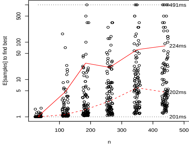
Figure 7: V5: Expected number of samples k^* to observe S (log scale). The solid red line shows means k^* at each problem size; the dotted red line shows medians. The top and bottom lines mark k = 1000, 1 . Exclusive access times appear at the right.
