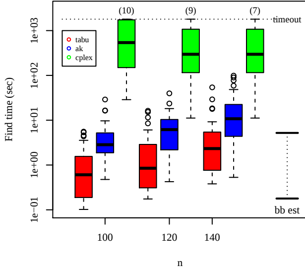
Figure 3: W2SAT software find times, and two estimates of median Blackbox find times (horizontal bars). Note the logarithmic y scale.
