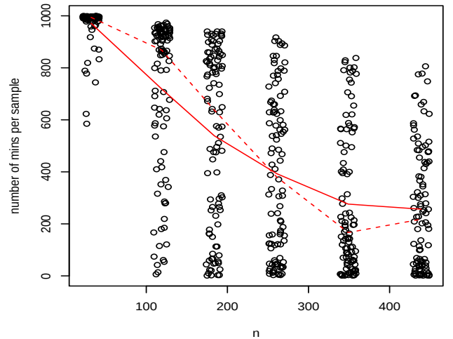
Figure 6: V5: Number of samples N holding the best answer S , in k = 1000 samples for each of 1000 inputs. The solid red line shows means and the dotted red line shows medians at each input size.
