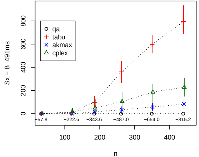
Figure 2: Differences between solution cost S_x in 491ms runtime, and best solution B for each input. Dotted lines connect means for each solver; vertical bars show the range of observations. The numbers at bottom are means \bar{B} for each problem size.
