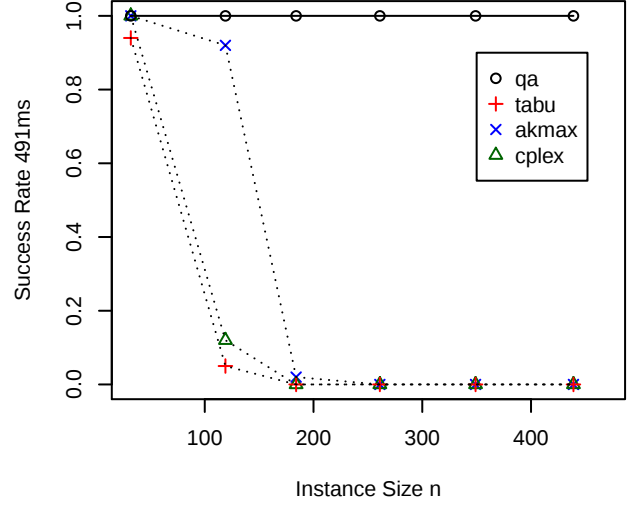
Figure 1: Success rates: proportion of best solutions found in 491ms CPU time (tabu, amax, cplex software) and exclusive access time (QA hardware).
