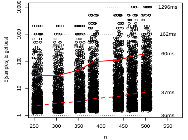
Figure 9: Expected number of samples to observe S . The solid red and dotted red lines show mean and medians over all inputs. The horizontal lines mark k = 1, 1000 , and 10,000 samples. Exclusive access times are shown on the right.
