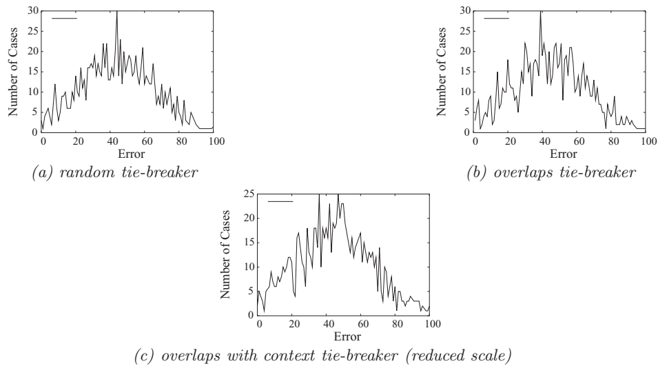
Fig. 10. Number of cases with error for each tie-breaker.
