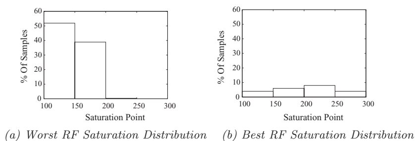
Fig. 11. Saturation occurs early for those cases where the RF error is bad.
