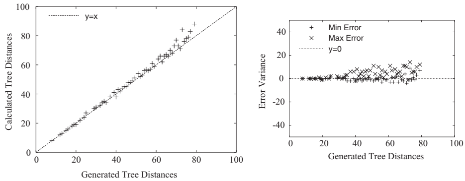
Fig. 3. Experimental results for 800 genes with expected edge length 10. Left : generated distance versus reconstructed distance; right : the variance of computed distances per generated distance.
