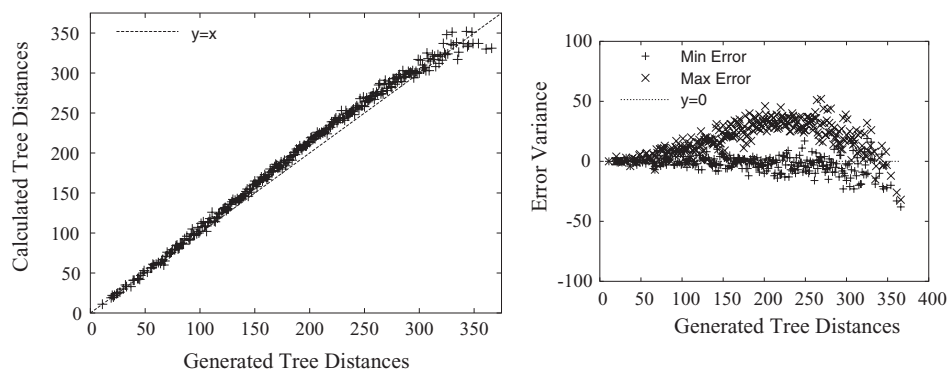
Fig. 7. Experimental results for 1,200 genes with expected edge length 20. Left : generated distance versus reconstructed distance; right : the variance of computed distances per generated distance.
