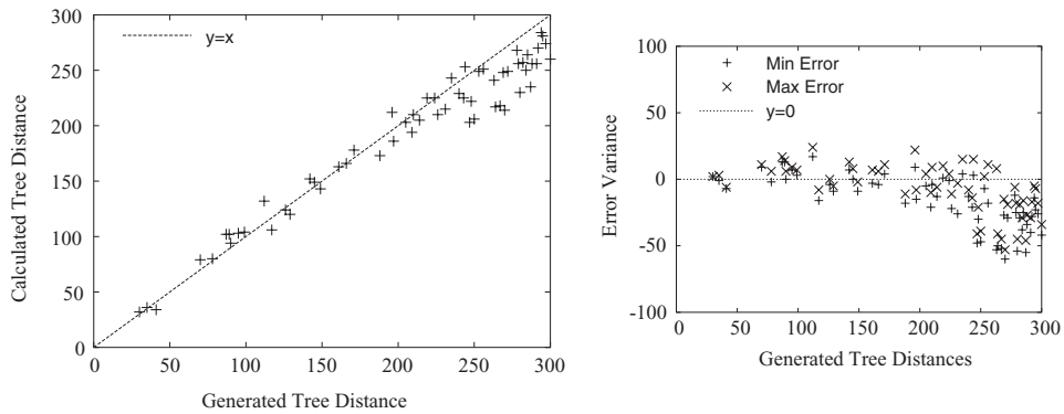
Fig. 5. Experimental results for 800 genes with expected edge length 40. Left : generated distance versus reconstructed distance; right : the variance of computed distances per generated distance.
