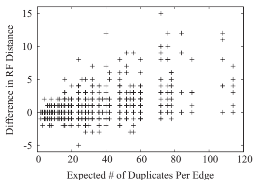
Fig. 9. The difference in RF distance between our method and the method without duplicates as a function of the number of duplicates on an edge.
