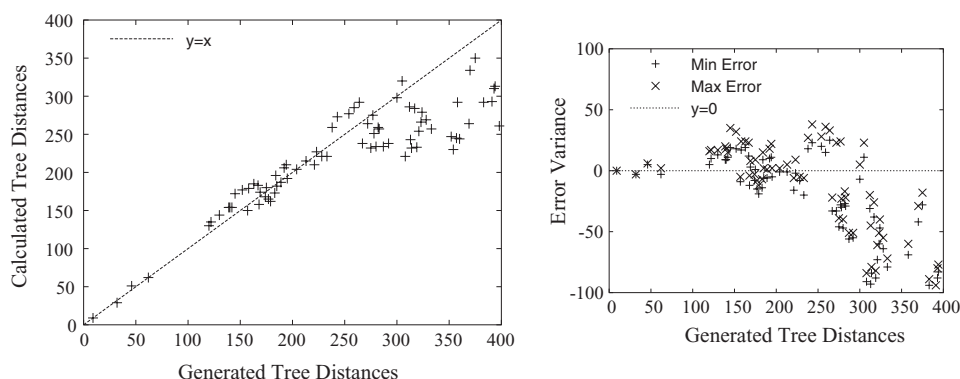
Fig. 6. Experimental results for 800 genes with expected edge length 60. Left : generated distance versus reconstructed distance; right : the variance of computed distances per generated distance.
