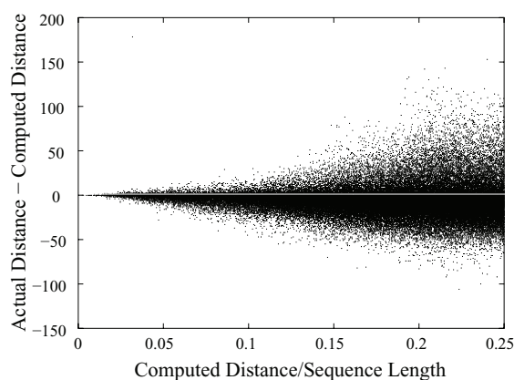
Fig. 12. Histogram of the error (actual distance—computed distance) as the ratio of the computed distance to the genome size increases.
