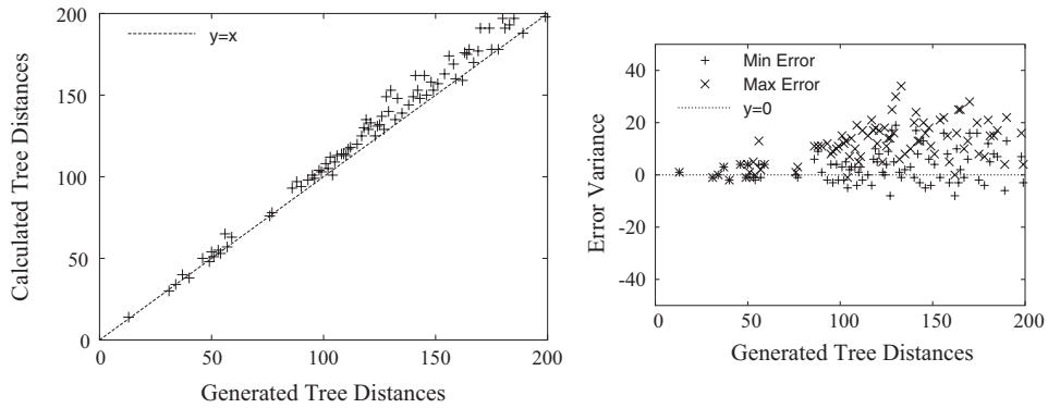
Fig. 4. Experimental results for 800 genes with expected edge length 20. Left : generated distance versus reconstructed distance; right : the variance of computed distances per generated distance.
